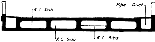
CROSS SECTION CELLULAR TYPE
